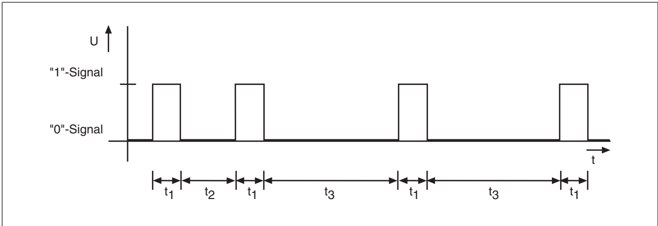
Timing diagram
