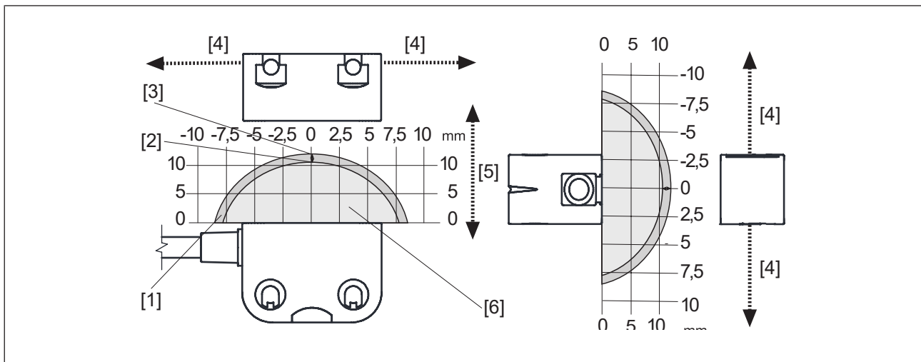
Fig.: Safety switches PSEN cs3.1n with actuator PSEN cs3.1
